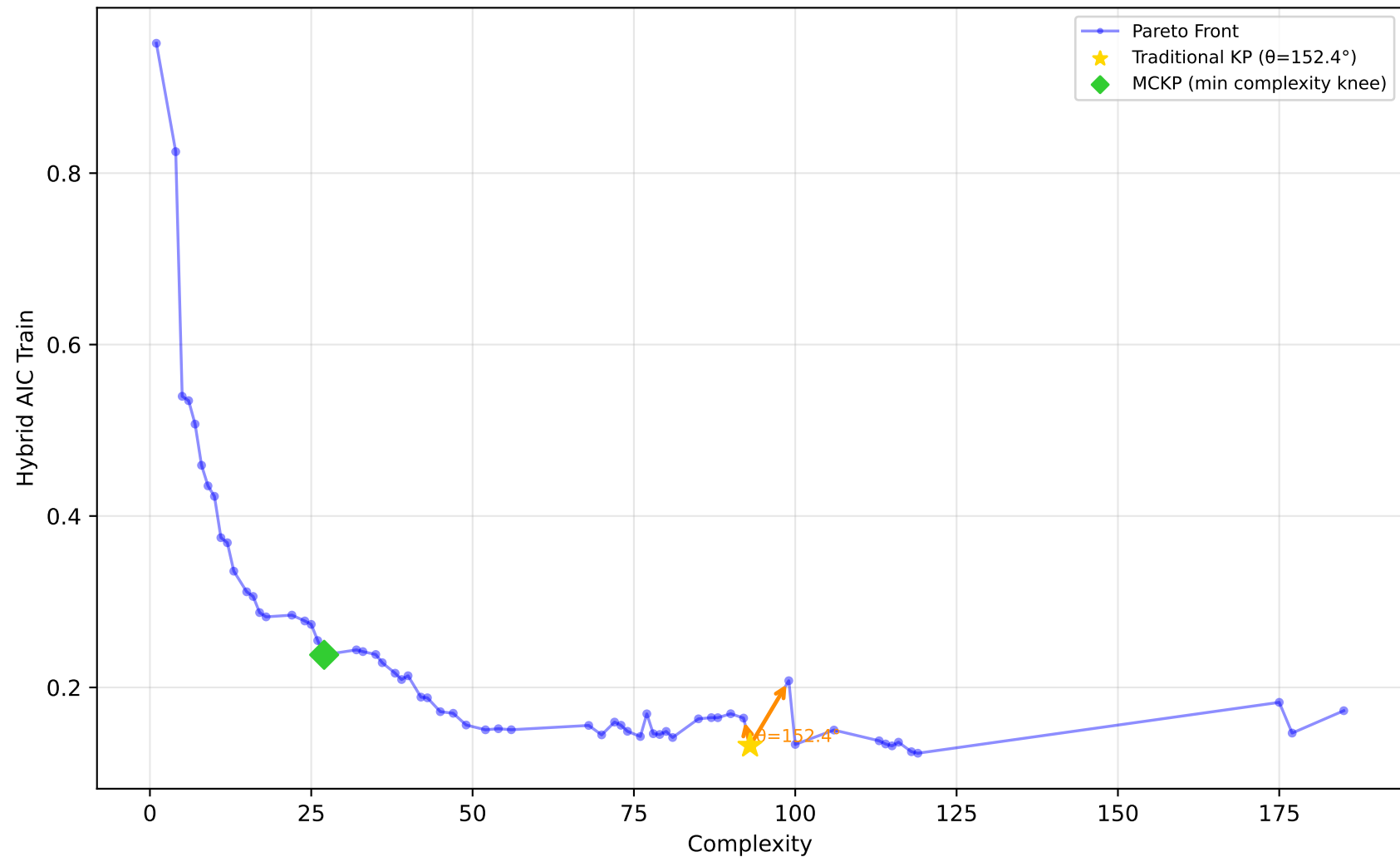
1028_SWD - Run 22 - SVP - Hybrid AIC Train \lambda_1=0.60, \lambda_2=0.00, \lambda_3=0.00 | Difficulty: 1.00 | Method: hmr
