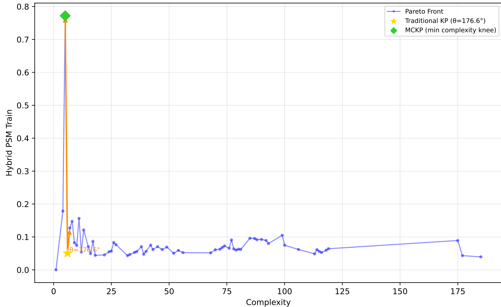
1028_SWD - Run 22 - SVP - Hybrid PSM Train \lambda_1=0.60, \lambda_2=0.00, \lambda_3=0.00 | Difficulty: 1.00 | Method: hmr
