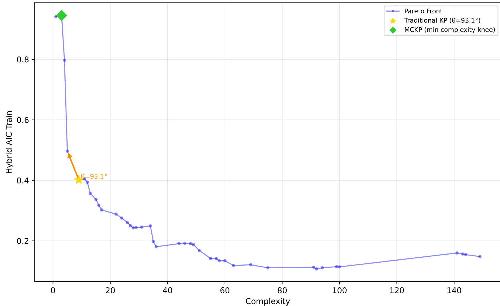
1028_SWD - Run 23 - MVP - Hybrid AIC Train \lambda_1=0.00, \lambda_2=0.00, \lambda_3=0.00 | Difficulty: 1.00 | Method: hmr
