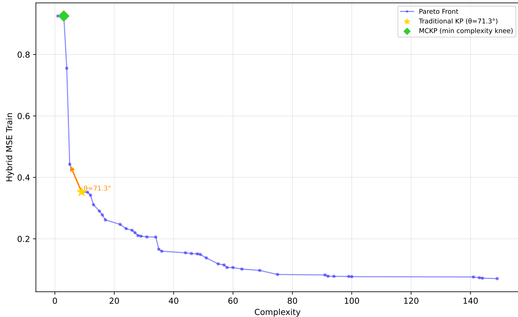
1028_SWD - Run 23 - MVP - Hybrid MSE Train \lambda_1=0.00, \lambda_2=0.00, \lambda_3=0.00 | Difficulty: 1.00 | Method: hmr
