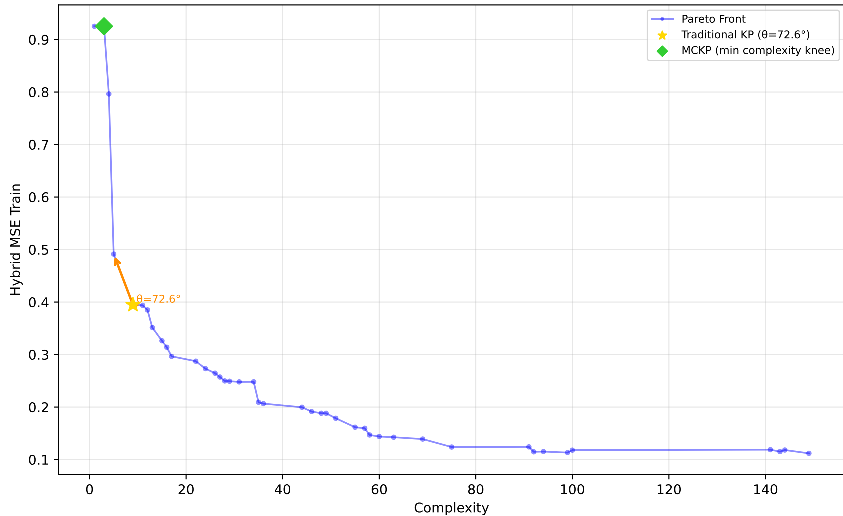
1028_SWD - Run 23 - MVP - Hybrid MSE Train \lambda_1=0.60, \lambda_2=0.00, \lambda_3=0.00 | Difficulty: 1.00 | Method: hmr
