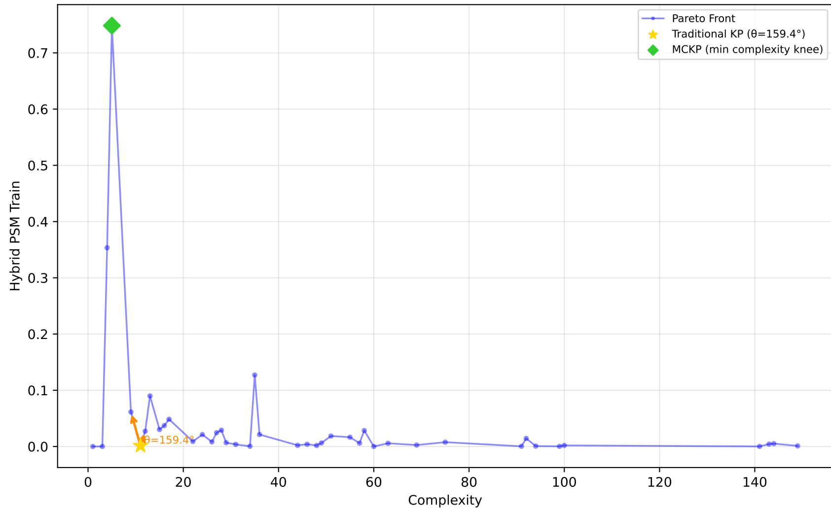
1028_SWD - Run 23 - MVP - Hybrid PSM Train \lambda_1=0.00, \lambda_2=0.00, \lambda_3=0.00 | Difficulty: 1.00 | Method: hmr
