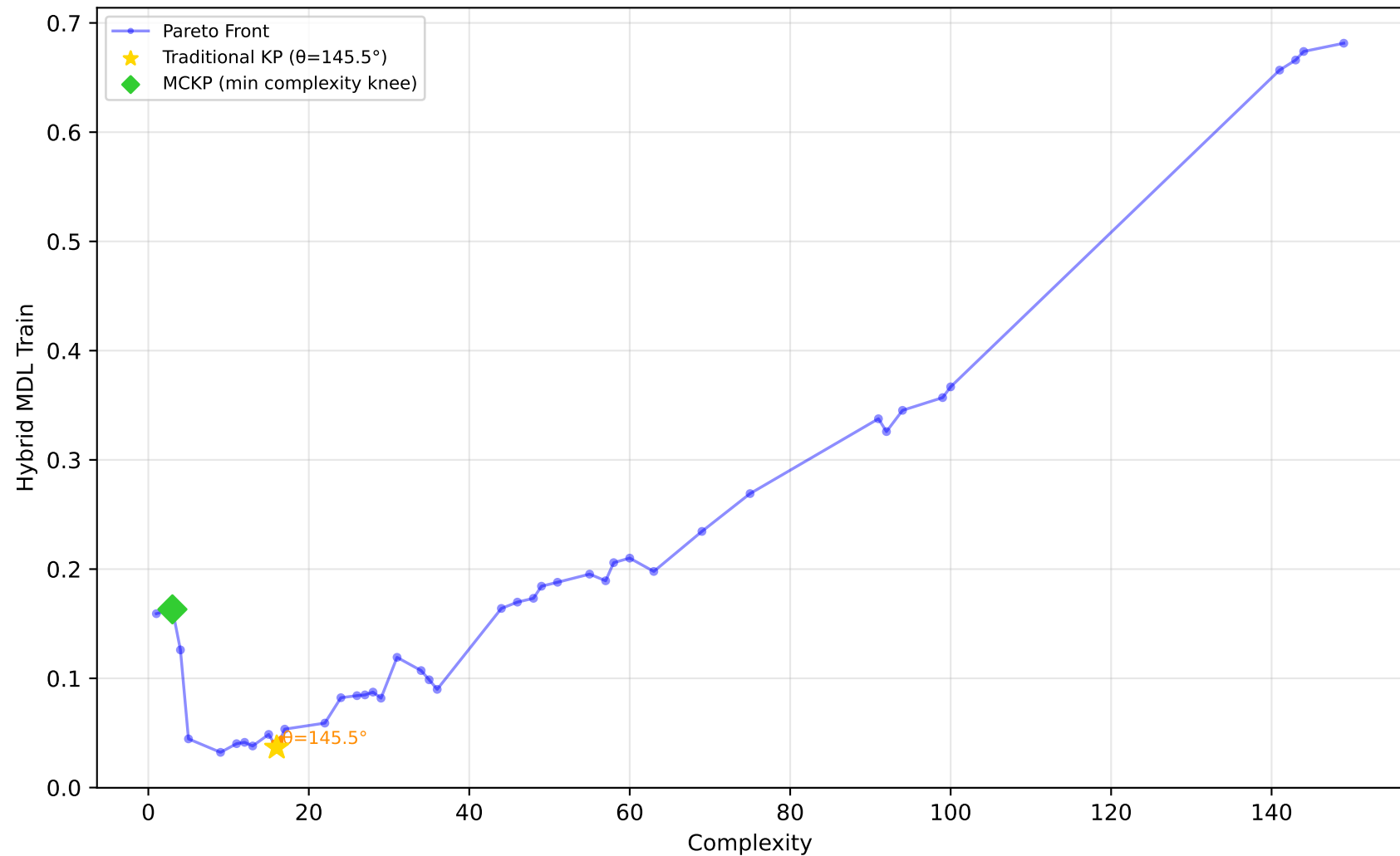
1028_SWD - Run 23 - SVP - Hybrid MDL Train \lambda_1=0.00, \lambda_2=0.60, \lambda_3=0.00 | Difficulty: 1.00 | Method: hmr
