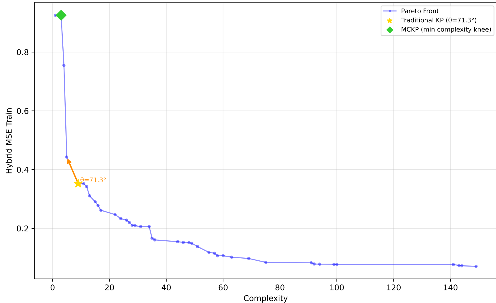
1028_SWD - Run 23 - SVP - Hybrid MSE Train \lambda_1=0.00, \lambda_2=0.60, \lambda_3=0.00 | Difficulty: 1.00 | Method: hmr
