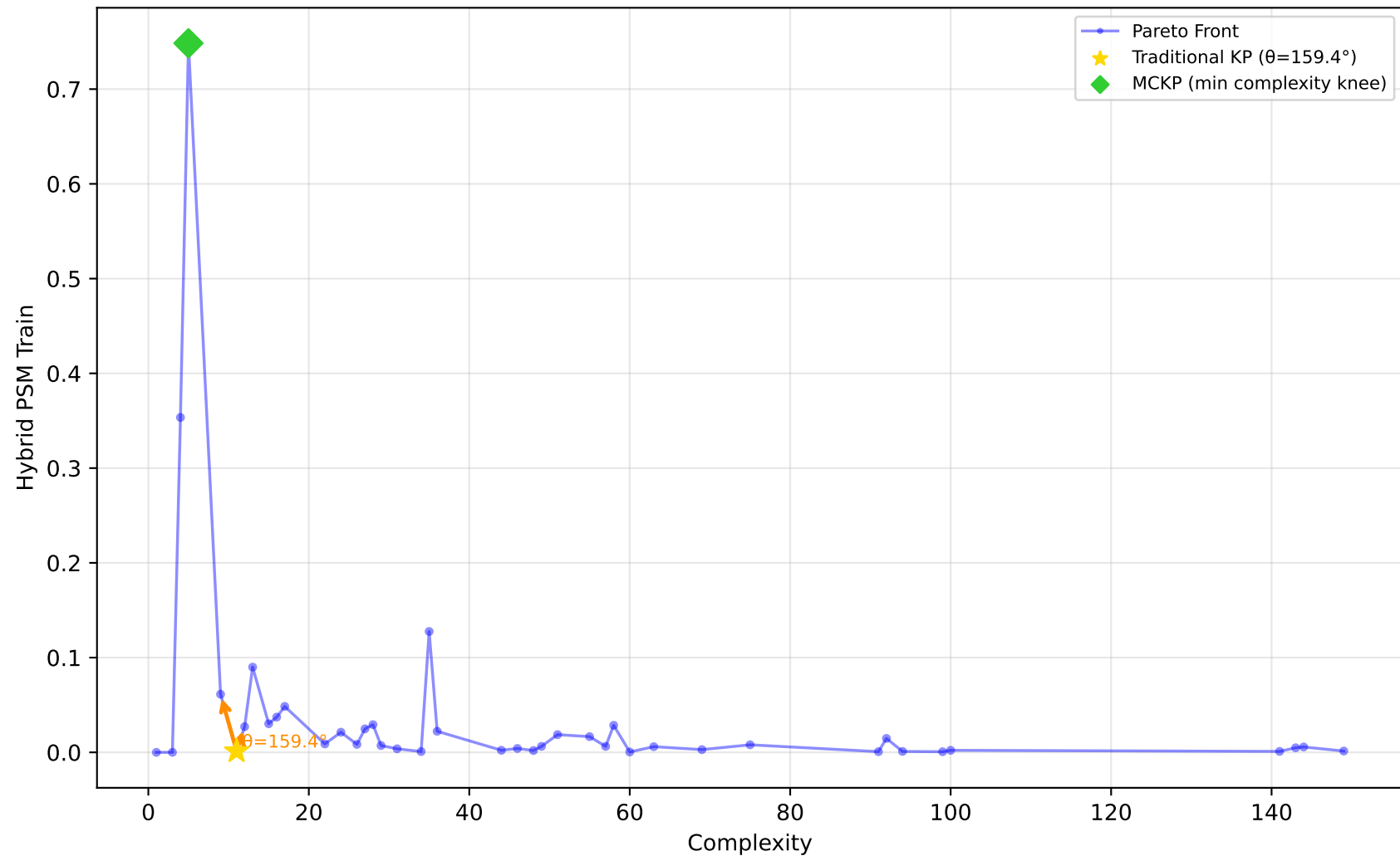
1028_SWD - Run 23 - SVP - Hybrid PSM Train \lambda_1=0.00, \lambda_2=0.60, \lambda_3=0.00 | Difficulty: 1.00 | Method: hmr
