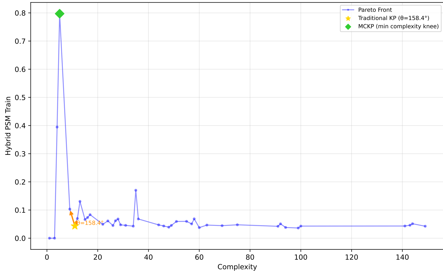
1028_SWD - Run 23 - SVP - Hybrid PSM Train \lambda_1=0.60, \lambda_2=0.00, \lambda_3=0.00 | Difficulty: 1.00 | Method: hmr
