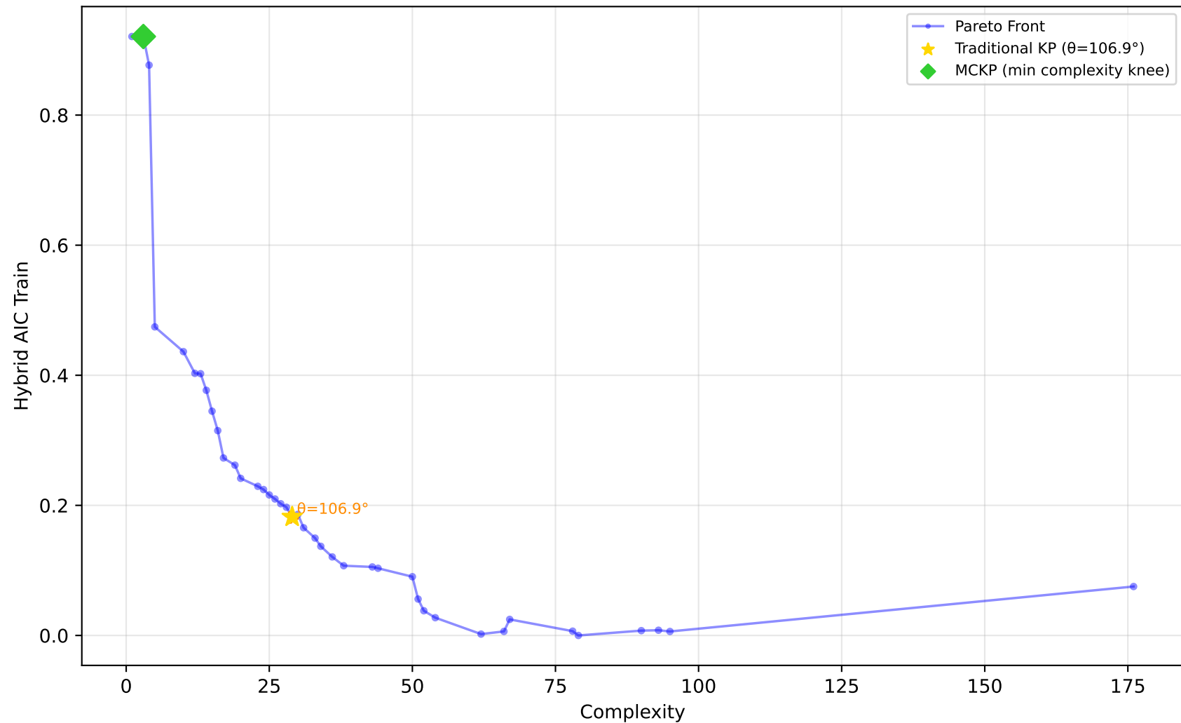
1028_SWD - Run 24 - MVP - Hybrid AIC Train \lambda_1=0.00, \lambda_2=0.00, \lambda_3=0.00 | Difficulty: 1.00 | Method: hmr
