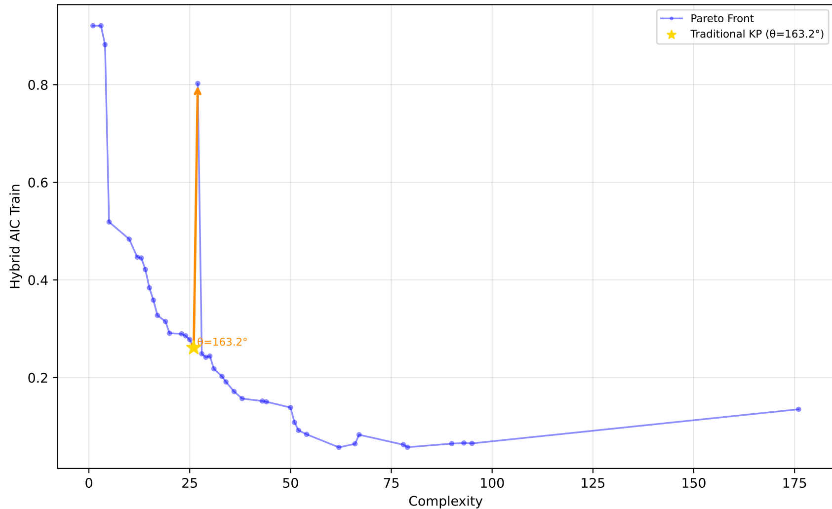
1028_SWD - Run 24 - MVP - Hybrid AIC Train \lambda_1=0.60, \lambda_2=0.00, \lambda_3=0.00 | Difficulty: 1.00 | Method: hmr
