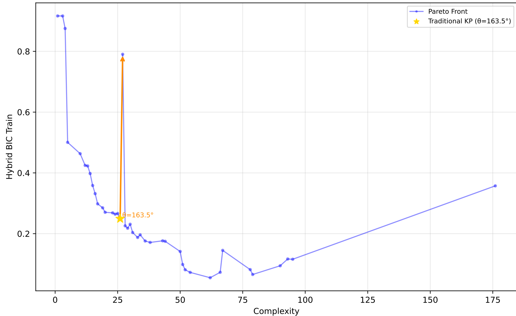
1028_SWD - Run 24 - MVP - Hybrid BIC Train \lambda_1=0.60, \lambda_2=0.00, \lambda_3=0.00 | Difficulty: 1.00 | Method: hmr
