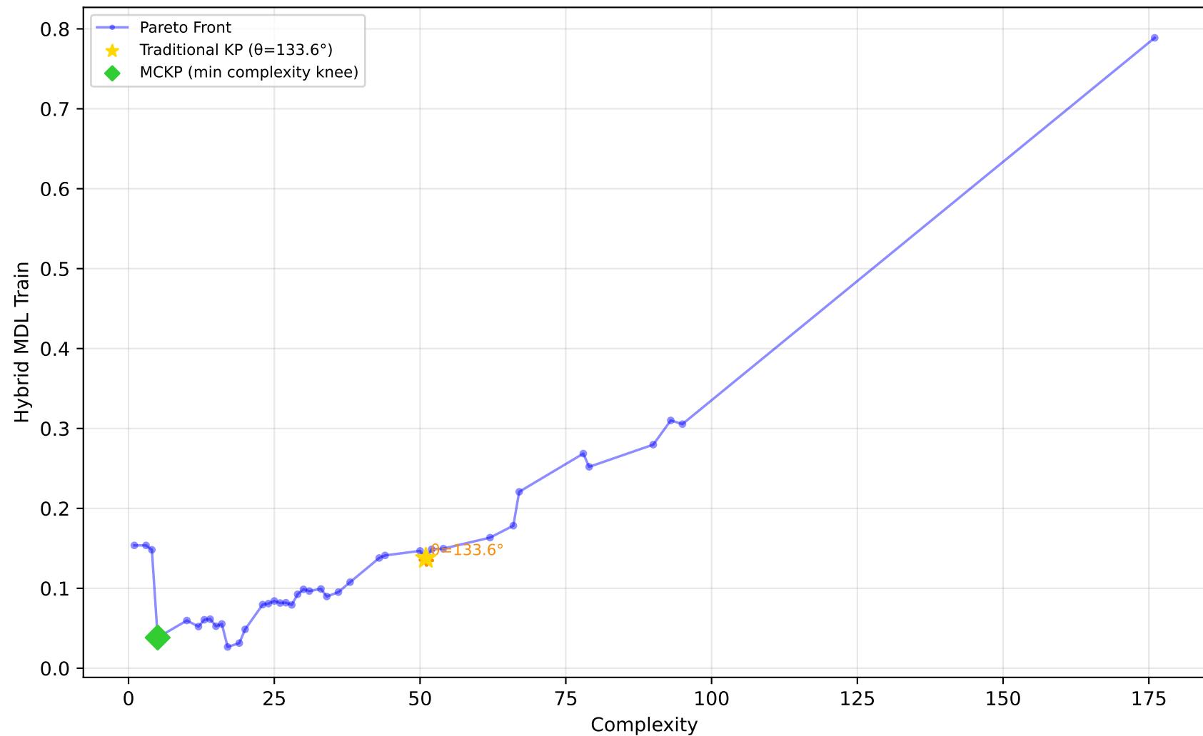
1028_SWD - Run 24 - MVP - Hybrid MDL Train \lambda_1=0.00, \lambda_2=0.00, \lambda_3=0.00 | Difficulty: 1.00 | Method: hmr
