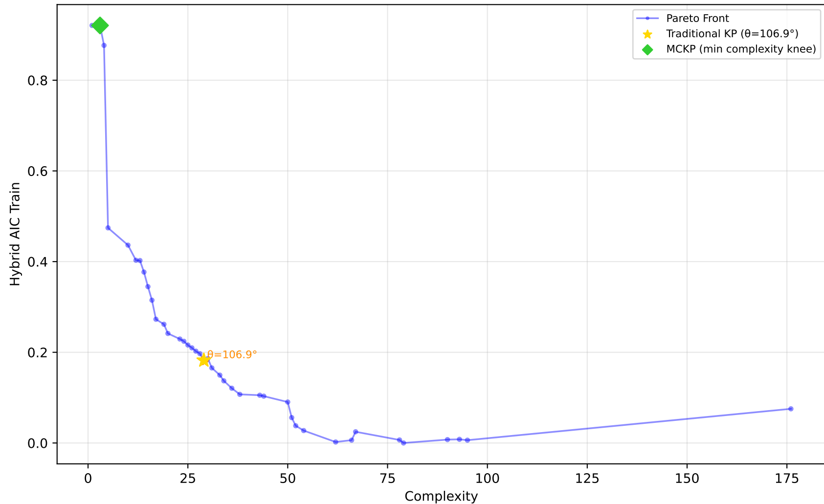
1028_SWD - Run 24 - SVP - Hybrid AIC Train \lambda_1=0.00, \lambda_2=0.60, \lambda_3=0.00 | Difficulty: 1.00 | Method: hmr
