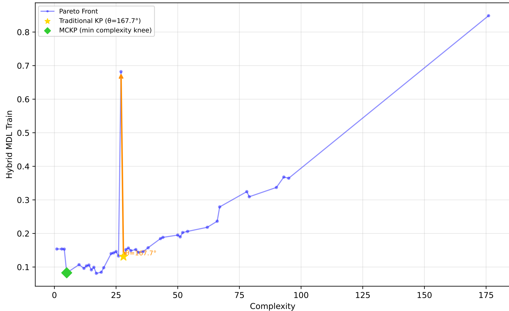
1028_SWD - Run 24 - SVP - Hybrid MDL Train \lambda_1=0.60, \lambda_2=0.00, \lambda_3=0.00 | Difficulty: 1.00 | Method: hmr
