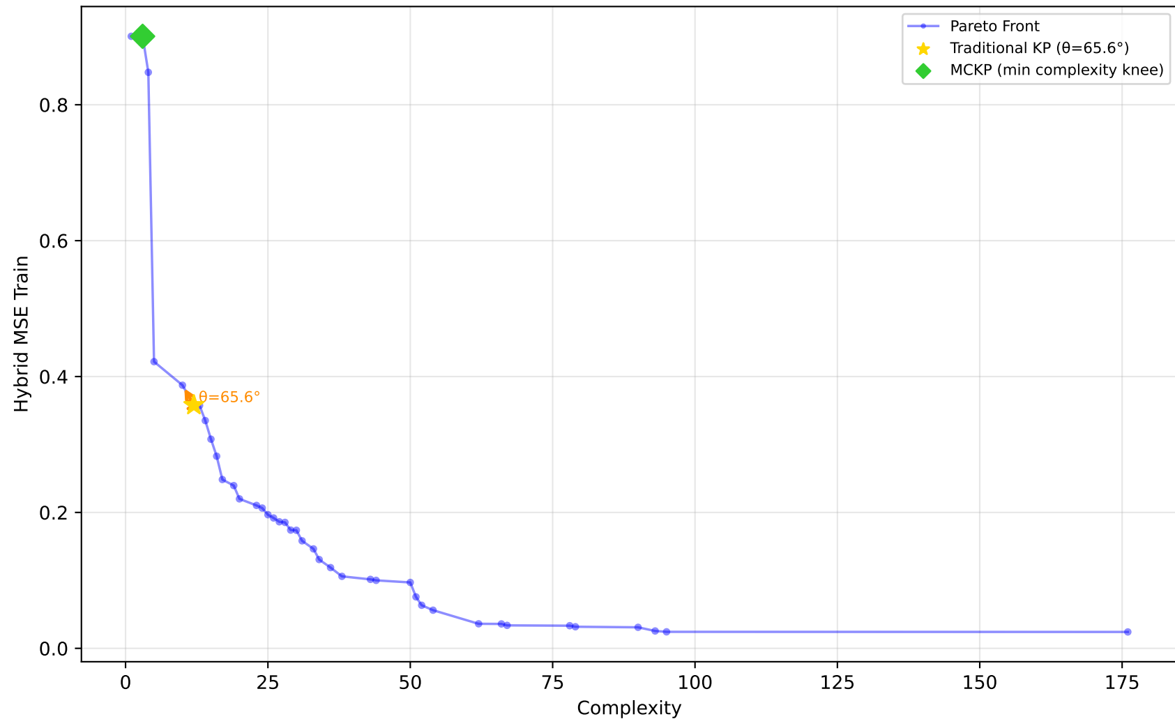
1028_SWD - Run 24 - SVP - Hybrid MSE Train \lambda_1=0.00, \lambda_2=0.60, \lambda_3=0.00 | Difficulty: 1.00 | Method: hmr
