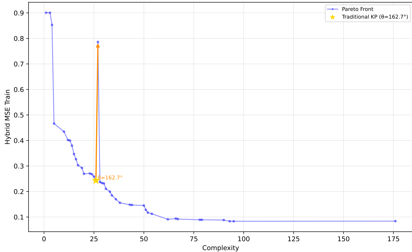
1028_SWD - Run 24 - SVP - Hybrid MSE Train \lambda_1=0.60, \lambda_2=0.00, \lambda_3=0.00 | Difficulty: 1.00 | Method: hmr
