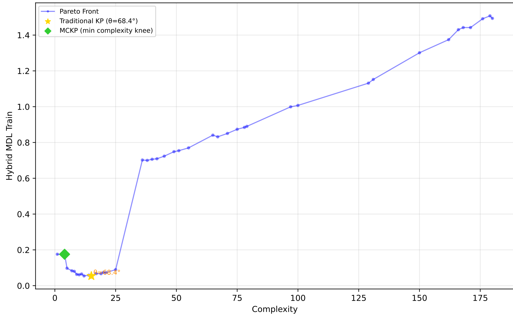
1028_SWD - Run 25 - MVP - Hybrid MDL Train \lambda_1=0.60, \lambda_2=0.00, \lambda_3=0.00 | Difficulty: 1.00 | Method: hmr
