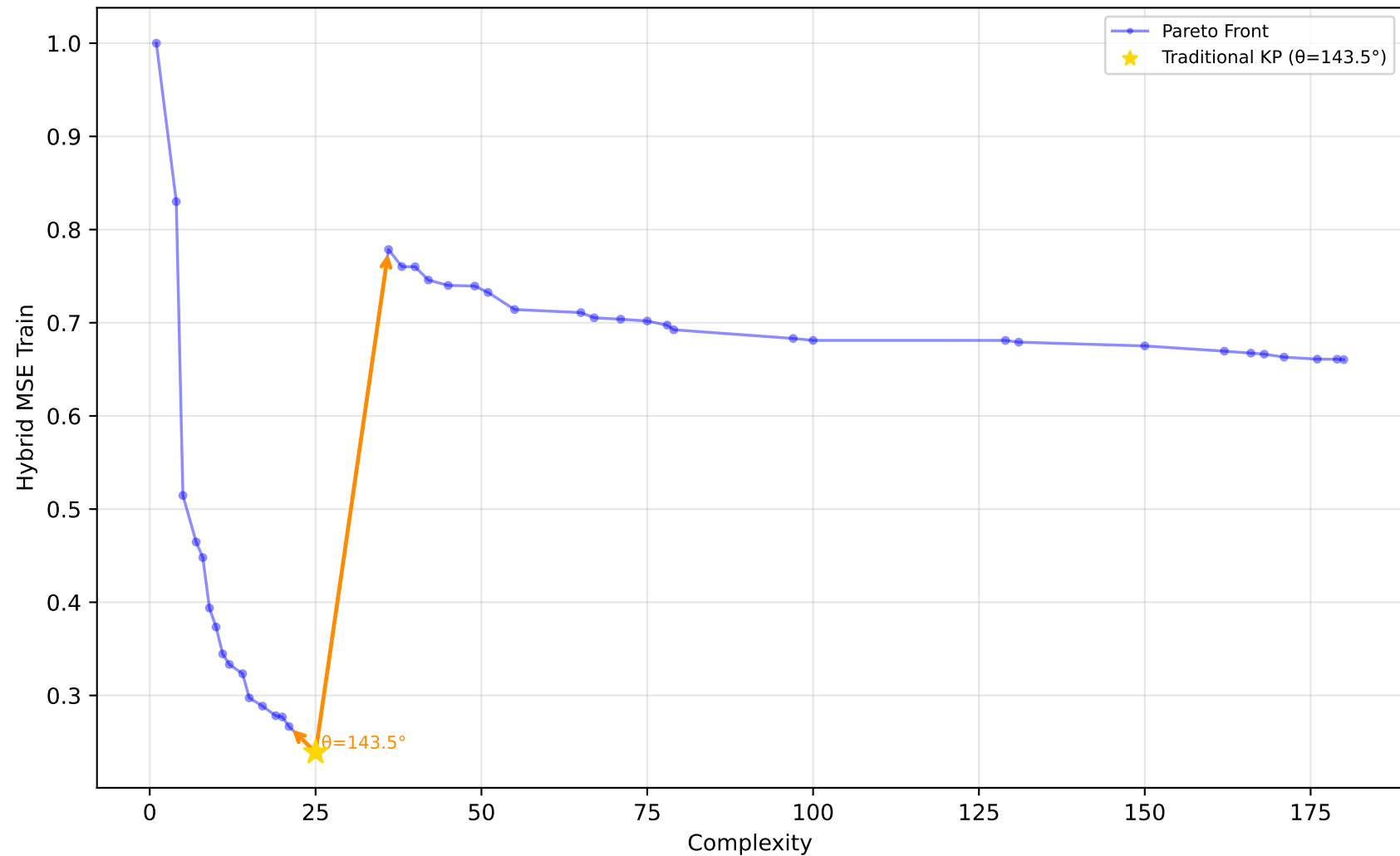
1028_SWD - Run 25 - MVP - Hybrid MSE Train \lambda_1=0.60, \lambda_2=0.00, \lambda_3=0.00 | Difficulty: 1.00 | Method: hmr
