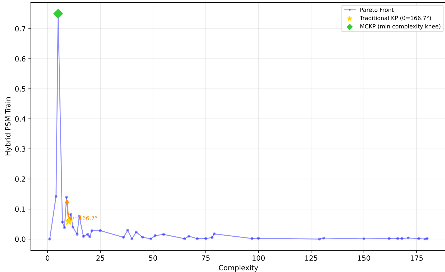
1028_SWD - Run 25 - MVP - Hybrid PSM Train \lambda_1=0.00, \lambda_2=0.00, \lambda_3=0.00 | Difficulty: 1.00 | Method: hmr
