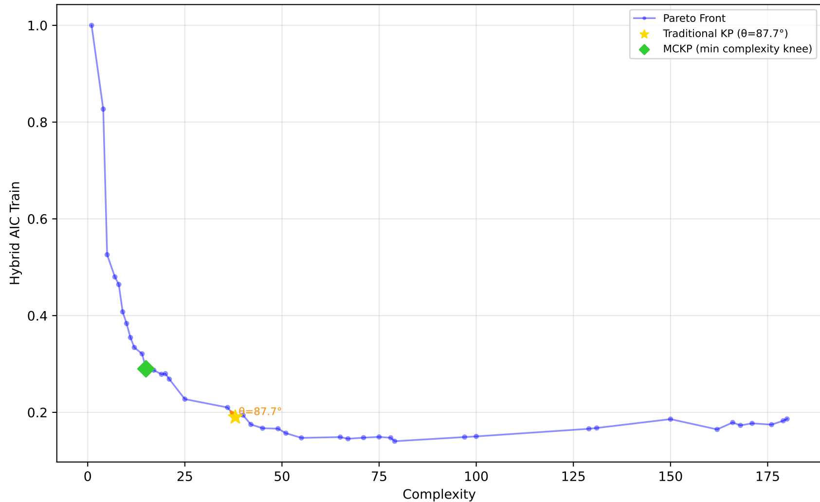
1028_SWD - Run 25 - SVP - Hybrid AIC Train \lambda_1=0.00, \lambda_2=0.60, \lambda_3=0.00 | Difficulty: 1.00 | Method: hmr
