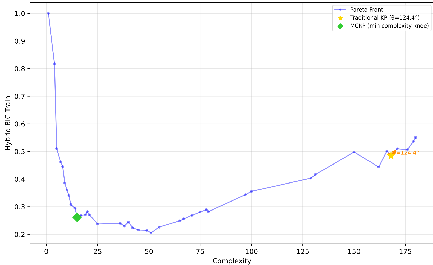
1028_SWD - Run 25 - SVP - Hybrid BIC Train \lambda_1=0.00, \lambda_2=0.60, \lambda_3=0.00 | Difficulty: 1.00 | Method: hmr
