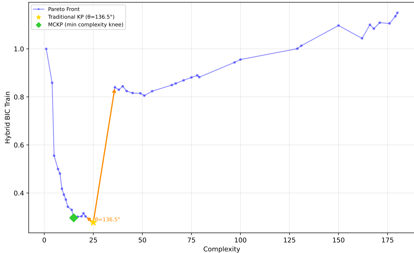
1028_SWD - Run 25 - SVP - Hybrid BIC Train \lambda_1=0.60, \lambda_2=0.00, \lambda_3=0.00 | Difficulty: 1.00 | Method: hmr
