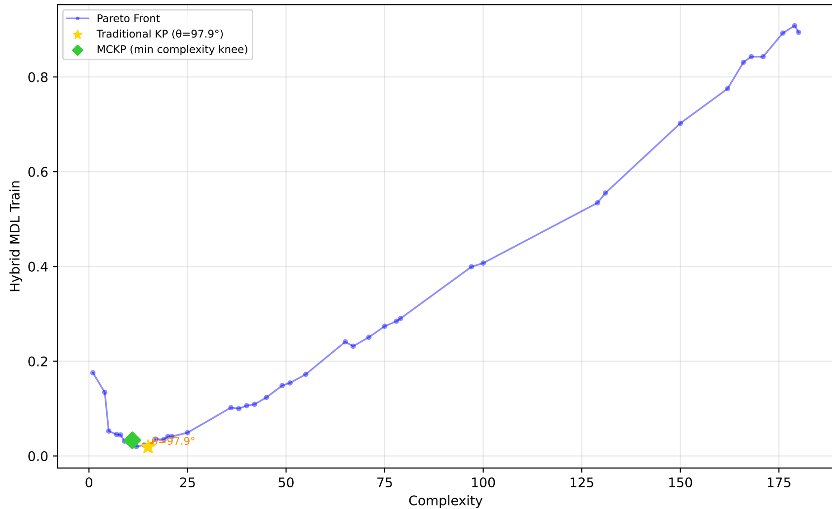
1028_SWD - Run 25 - SVP - Hybrid MDL Train \lambda_1=0.00, \lambda_2=0.60, \lambda_3=0.00 | Difficulty: 1.00 | Method: hmr
