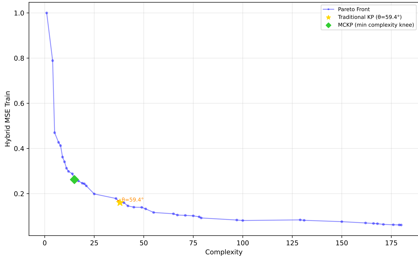
1028_SWD - Run 25 - SVP - Hybrid MSE Train \lambda_1=0.00, \lambda_2=0.60, \lambda_3=0.00 | Difficulty: 1.00 | Method: hmr
