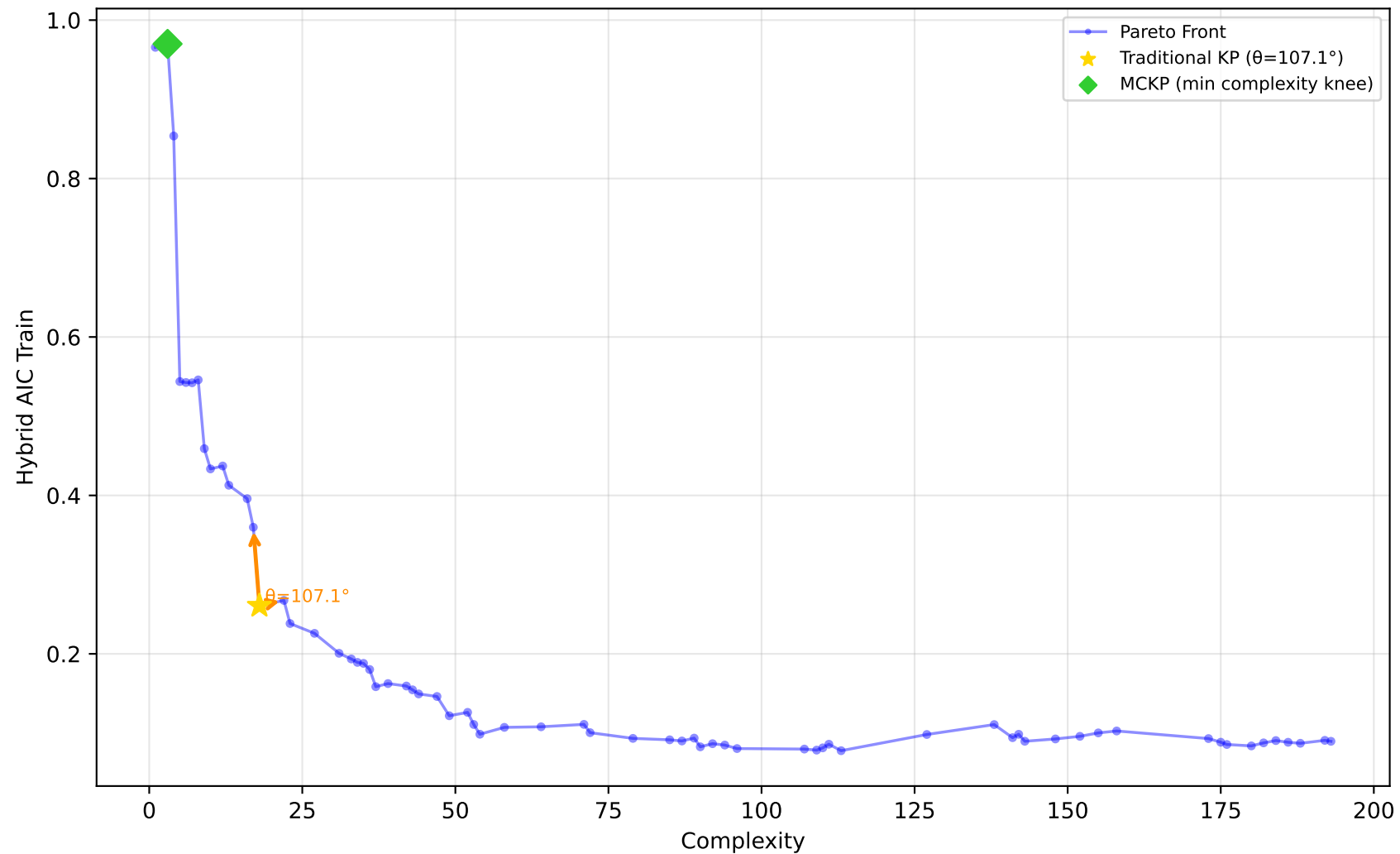
1028_SWD - Run 26 - MVP - Hybrid AIC Train \lambda_1=0.00, \lambda_2=0.00, \lambda_3=0.00 | Difficulty: 0.82 | Method: hmr
