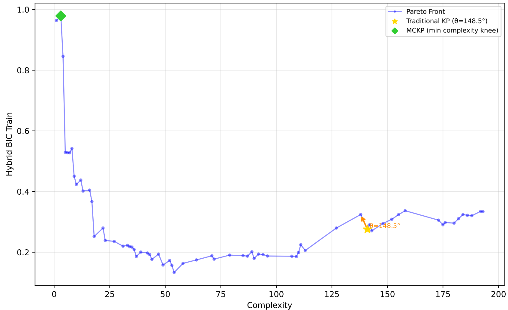
1028_SWD - Run 26 - MVP - Hybrid BIC Train \lambda_1=0.00, \lambda_2=0.00, \lambda_3=0.00 | Difficulty: 0.82 | Method: hmr
