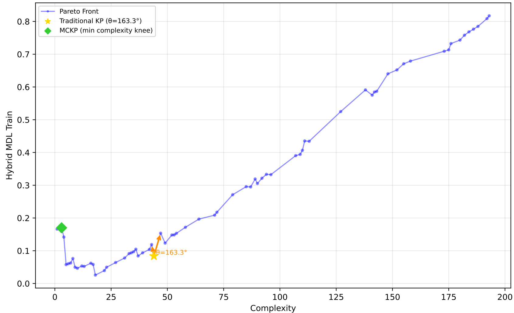
1028_SWD - Run 26 - MVP - Hybrid MDL Train \lambda_1=0.00, \lambda_2=0.00, \lambda_3=0.00 | Difficulty: 0.82 | Method: hmr
