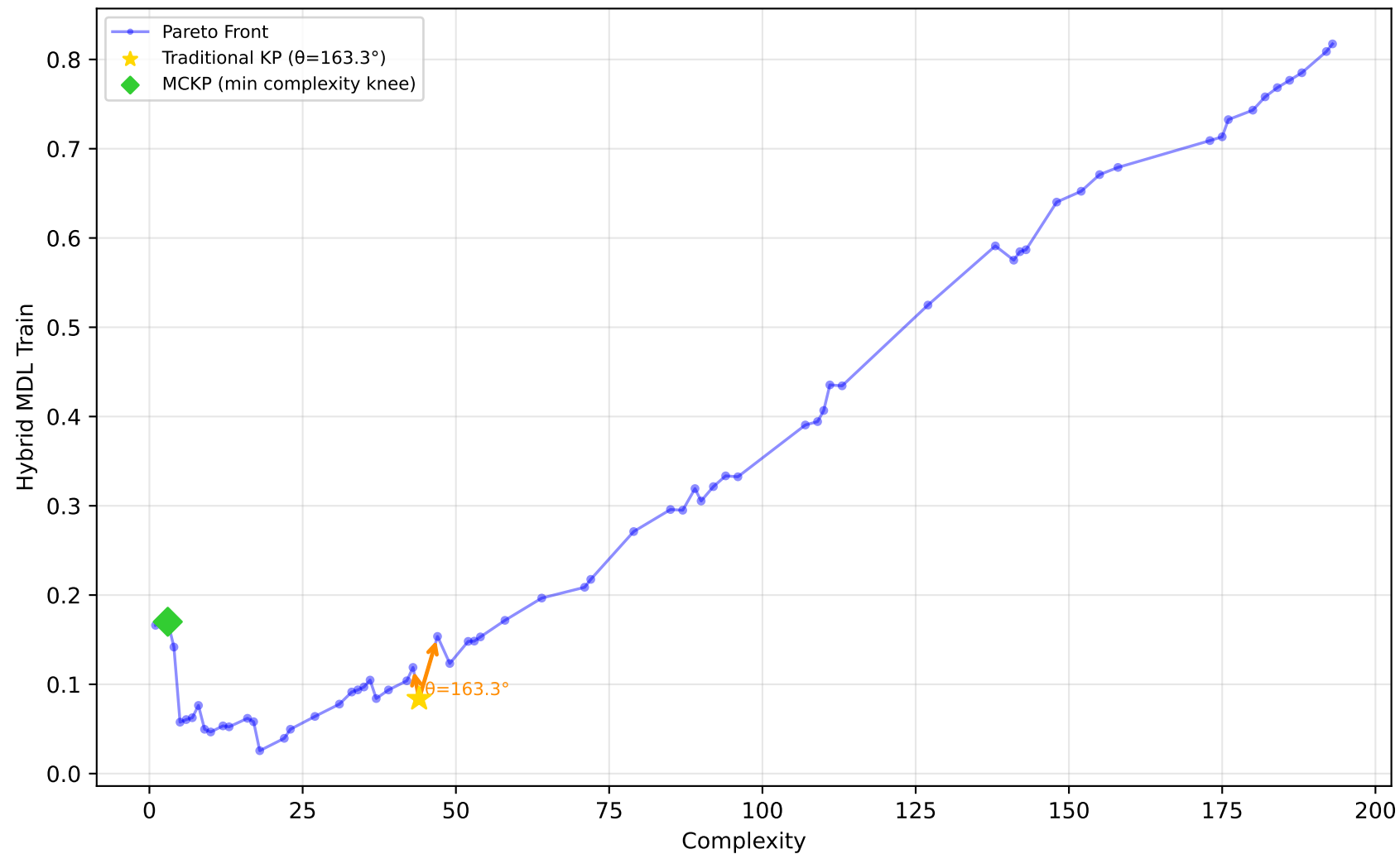
1028_SWD - Run 26 - SVP - Hybrid MDL Train \lambda_1=0.00, \lambda_2=0.60, \lambda_3=0.00 | Difficulty: 0.82 | Method: hmr
