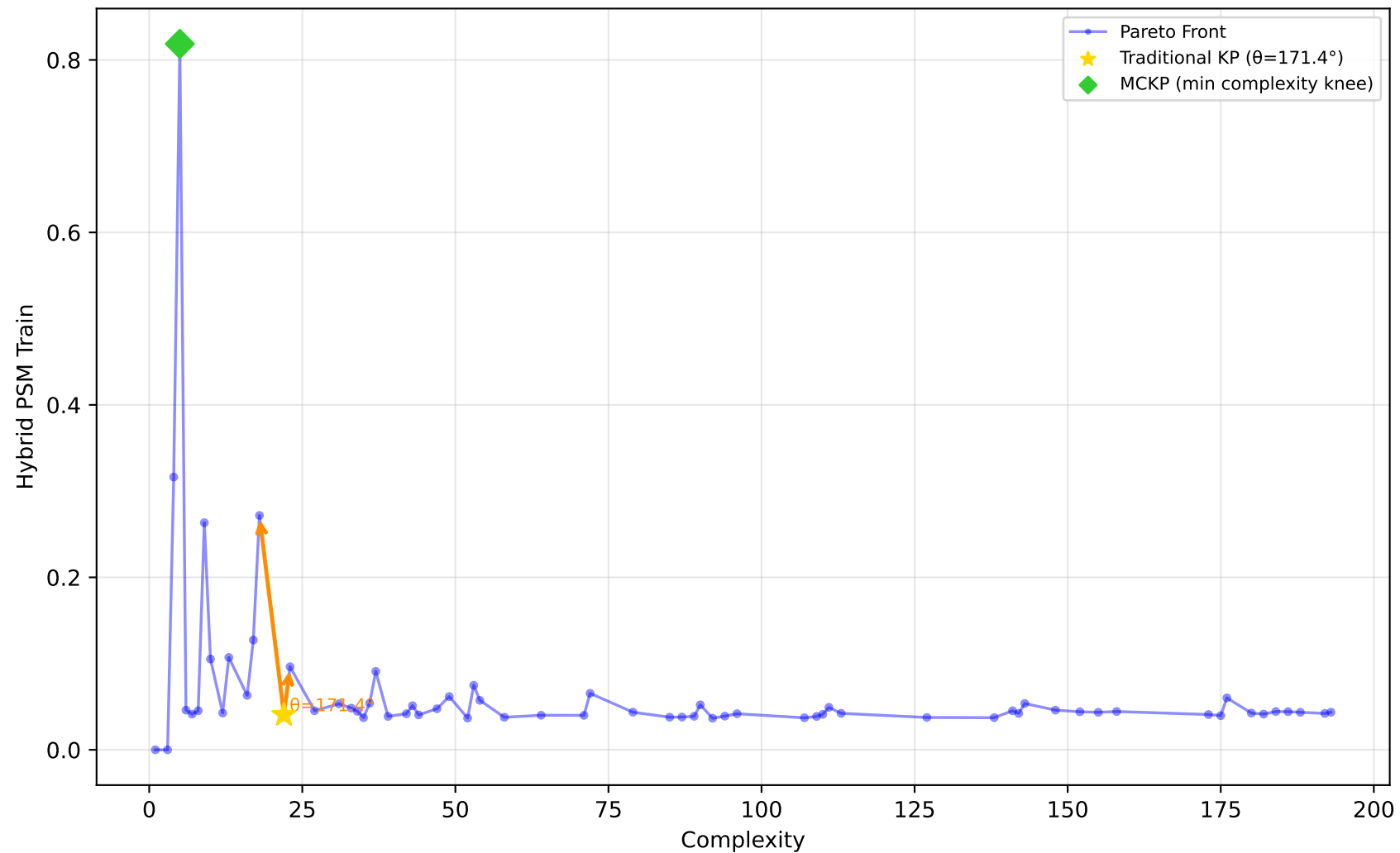
1028_SWD - Run 26 - SVP - Hybrid PSM Train \lambda_1=0.60, \lambda_2=0.00, \lambda_3=0.00 | Difficulty: 0.82 | Method: hmr
