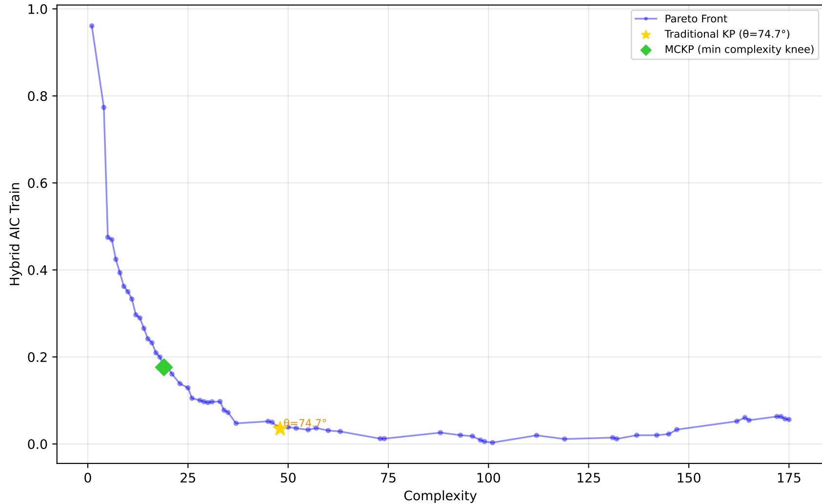
1028_SWD - Run 27 - MVP - Hybrid AIC Train \lambda_1=0.00, \lambda_2=0.00, \lambda_3=0.00 | Difficulty: 1.00 | Method: hmr
