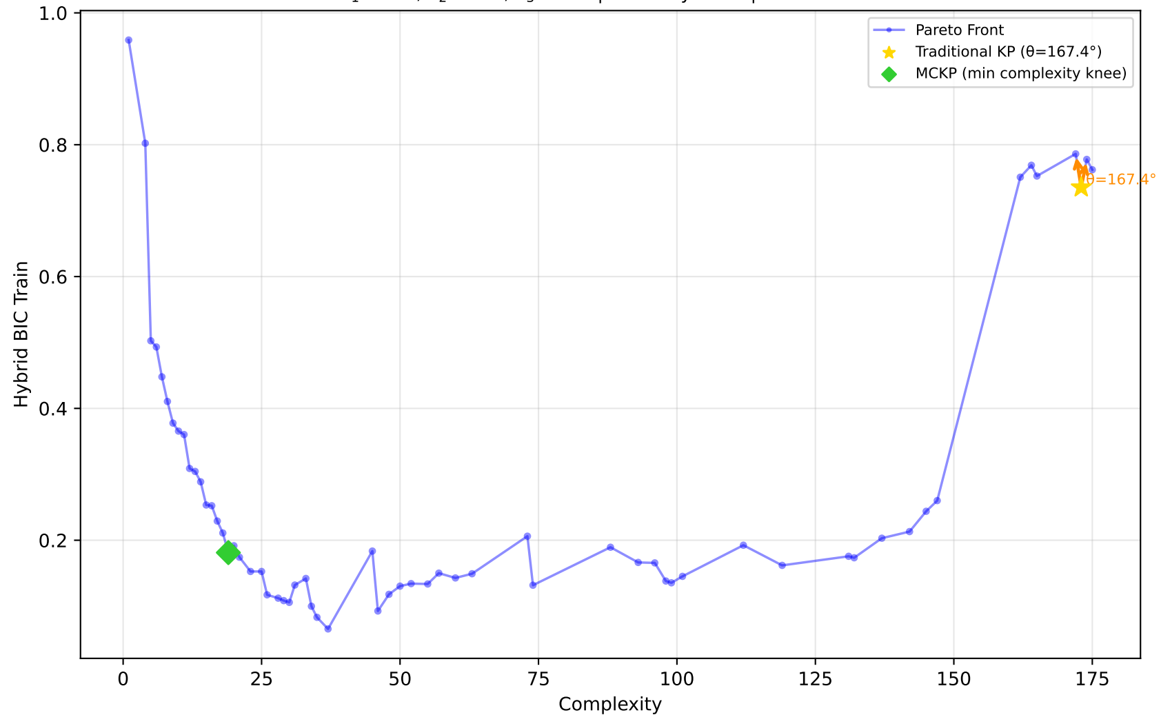
1028_SWD - Run 27 - MVP - Hybrid BIC Train \lambda_1=0.60, \lambda_2=0.00, \lambda_3=0.00 | Difficulty: 1.00 | Method: hmr
