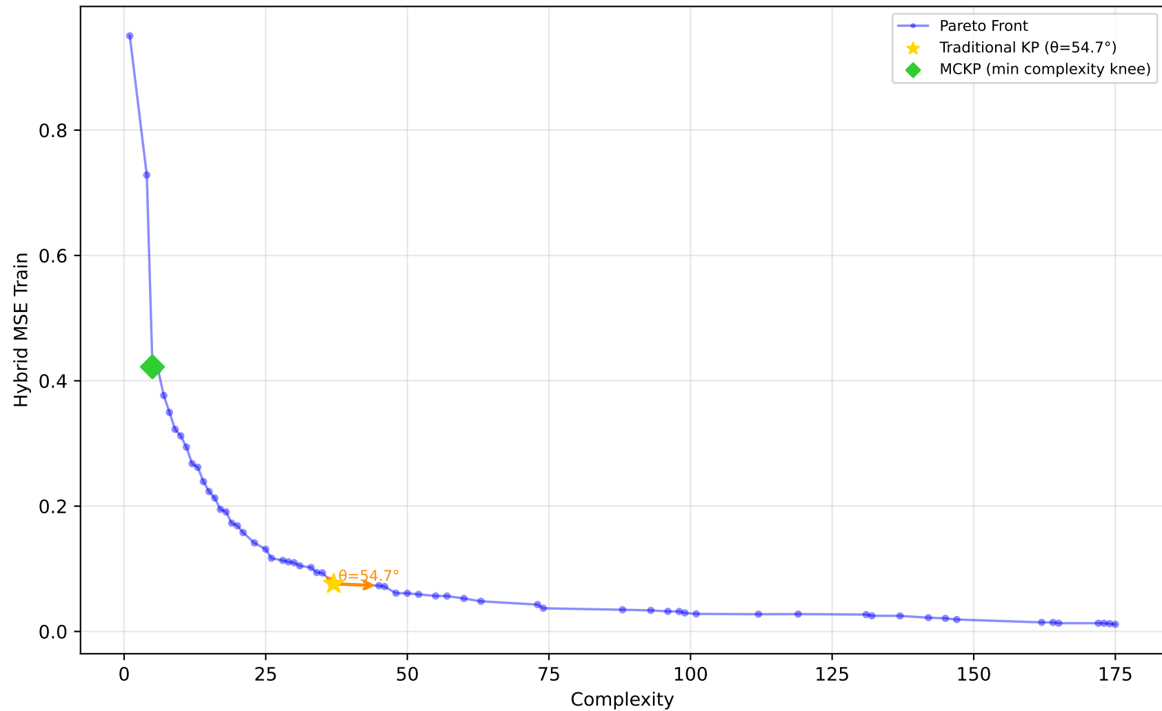
1028_SWD - Run 27 - MVP - Hybrid MSE Train \lambda_1=0.00, \lambda_2=0.00, \lambda_3=0.00 | Difficulty: 1.00 | Method: hmr
