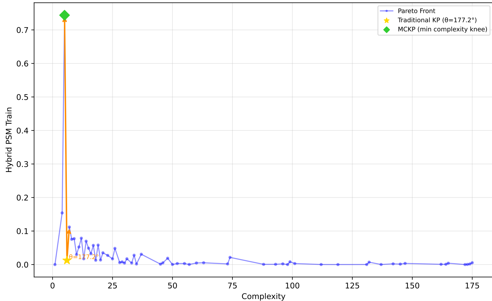
1028_SWD - Run 27 - MVP - Hybrid PSM Train \lambda_1=0.00, \lambda_2=0.00, \lambda_3=0.00 | Difficulty: 1.00 | Method: hmr
