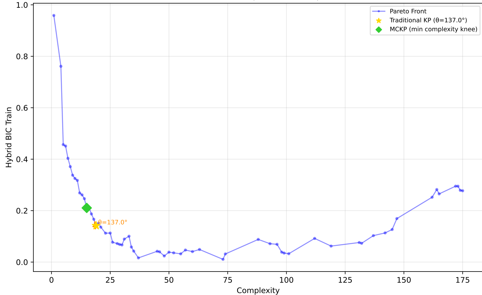
1028_SWD - Run 27 - SVP - Hybrid BIC Train \lambda_1=0.00, \lambda_2=0.60, \lambda_3=0.00 | Difficulty: 1.00 | Method: hmr
