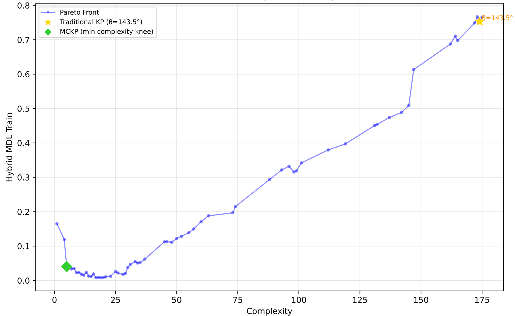
1028_SWD - Run 27 - SVP - Hybrid MDL Train \lambda_1=0.00, \lambda_2=0.60, \lambda_3=0.00 | Difficulty: 1.00 | Method: hmr
