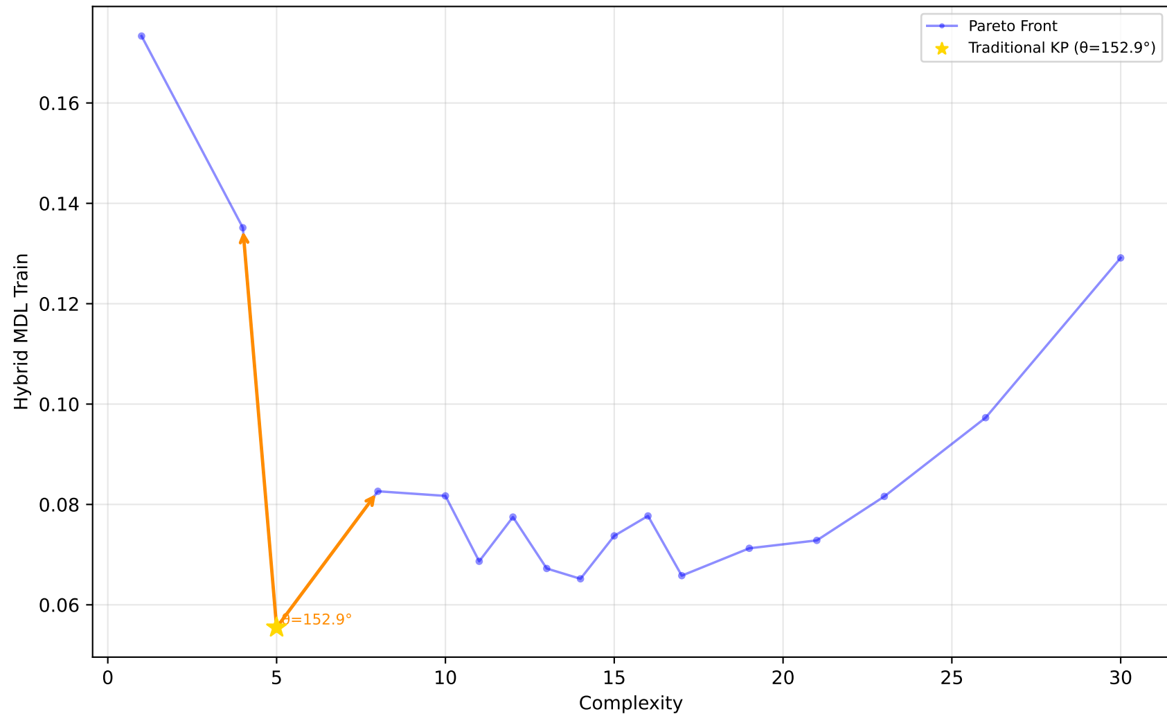
1028_SWD - Run 28 - MVP - Hybrid MDL Train \lambda_1=0.00, \lambda_2=0.00, \lambda_3=0.00 | Difficulty: 1.00 | Method: hmr
