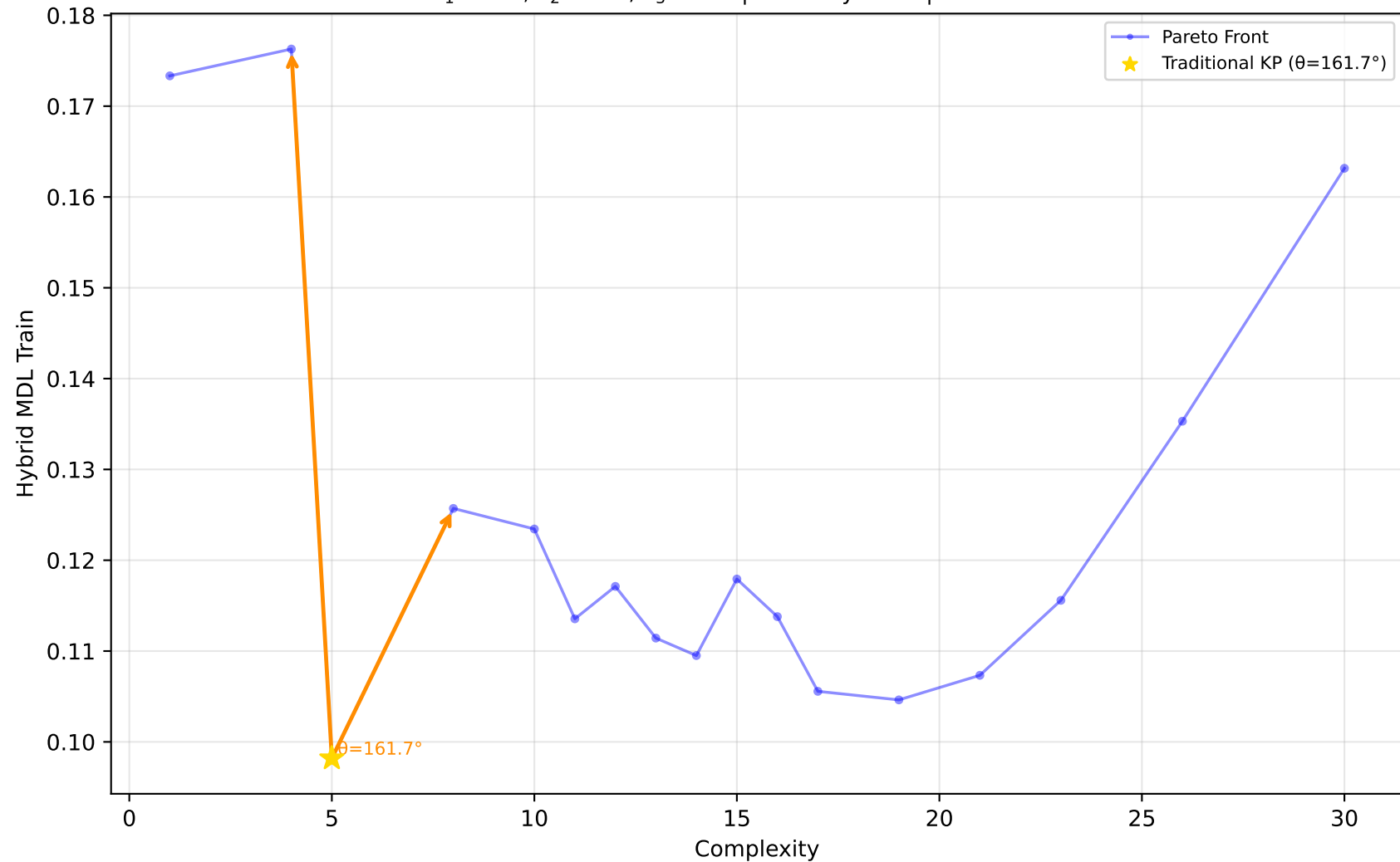
1028_SWD - Run 28 - MVP - Hybrid MDL Train \lambda_1=0.60, \lambda_2=0.00, \lambda_3=0.00 | Difficulty: 1.00 | Method: hmr
