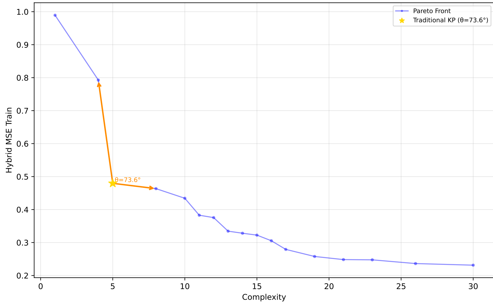
1028_SWD - Run 28 - MVP - Hybrid MSE Train \lambda_1=0.00, \lambda_2=0.00, \lambda_3=0.00 | Difficulty: 1.00 | Method: hmr
