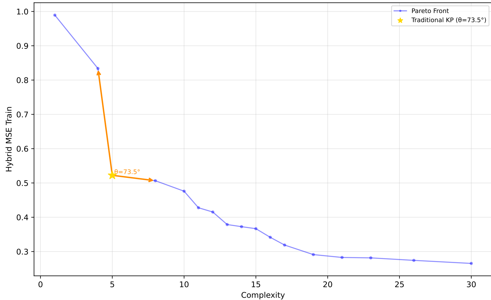
1028_SWD - Run 28 - MVP - Hybrid MSE Train \lambda_1=0.60, \lambda_2=0.00, \lambda_3=0.00 | Difficulty: 1.00 | Method: hmr
