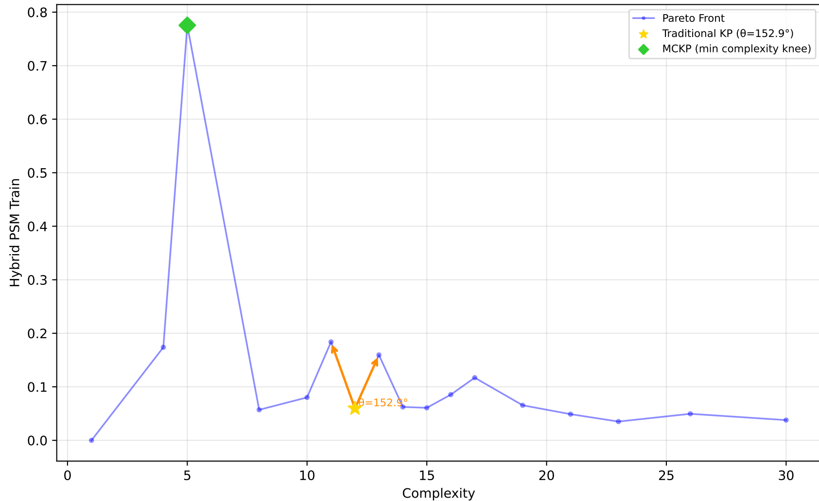
1028_SWD - Run 28 - MVP - Hybrid PSM Train \lambda_1=0.60, \lambda_2=0.00, \lambda_3=0.00 | Difficulty: 1.00 | Method: hmr
