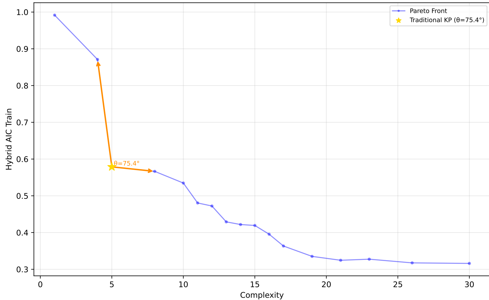
1028_SWD - Run 28 - SVP - Hybrid AIC Train \lambda_1=0.60, \lambda_2=0.00, \lambda_3=0.00 | Difficulty: 1.00 | Method: hmr
