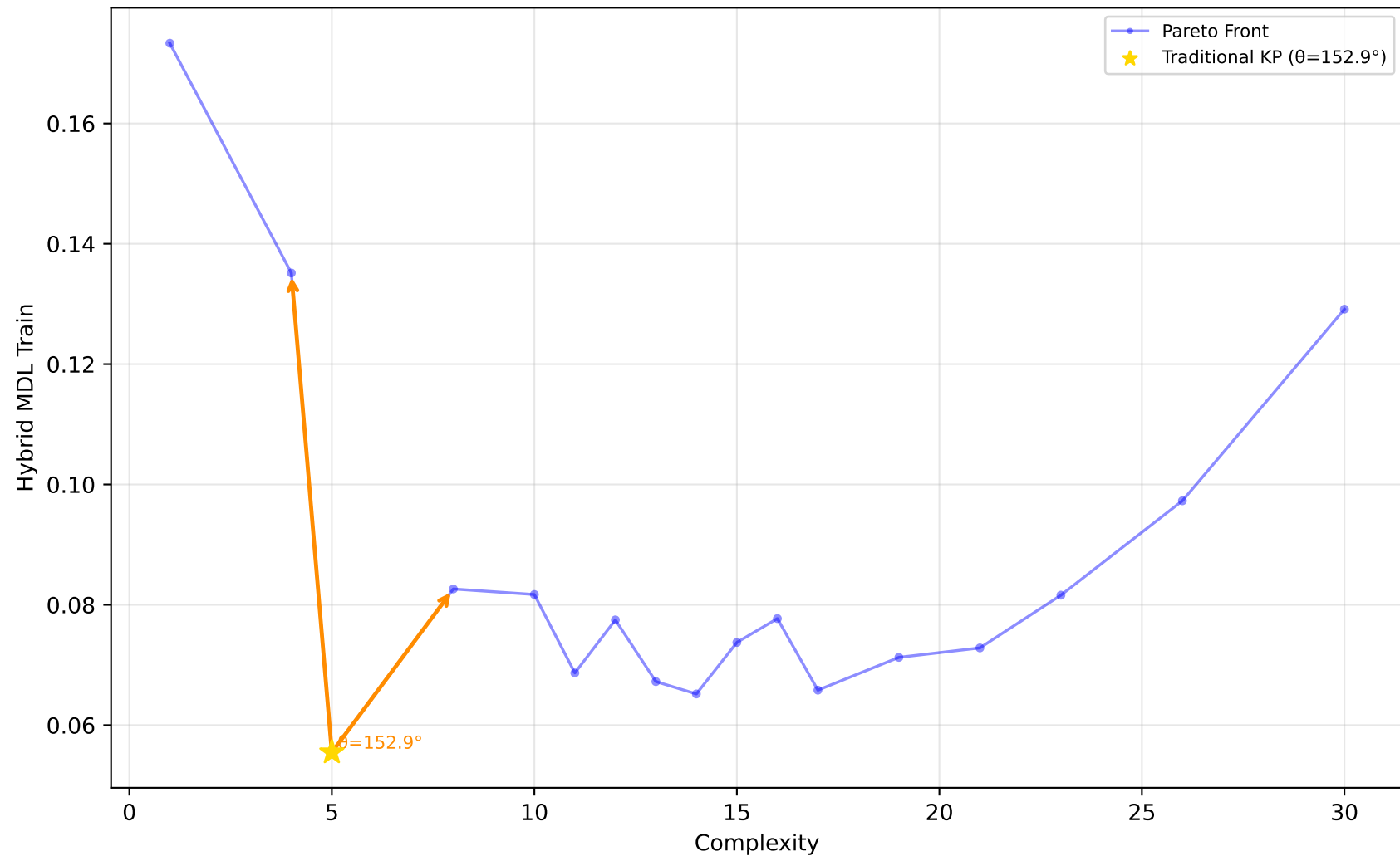
1028_SWD - Run 28 - SVP - Hybrid MDL Train \lambda_1=0.00, \lambda_2=0.60, \lambda_3=0.00 | Difficulty: 1.00 | Method: hmr
