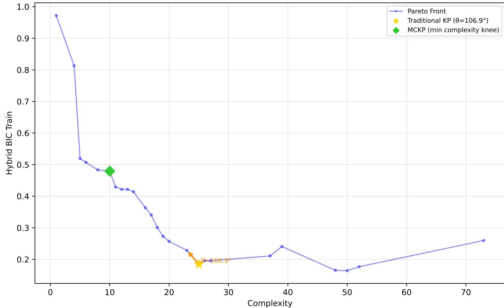
1028_SWD - Run 29 - MVP - Hybrid BIC Train \lambda_1=0.00, \lambda_2=0.00, \lambda_3=0.00 | Difficulty: 1.00 | Method: hmr
