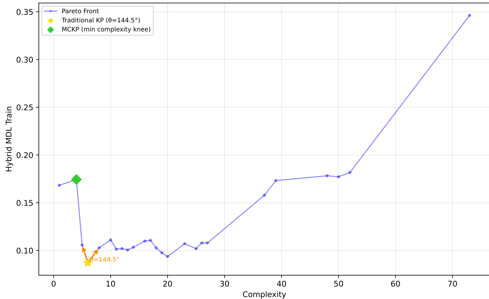
1028_SW_D - Run 29 - MVP - Hybrid MDL Train \lambda_1=0.60, \lambda_2=0.00, \lambda_3=0.00 | Difficulty: 1.00 | Method: hmr
