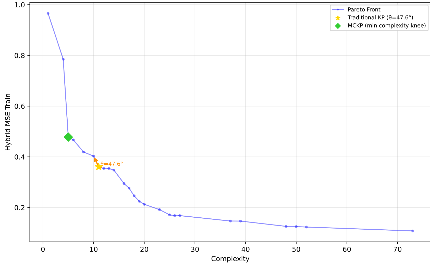
1028_SWD - Run 29 - MVP - Hybrid MSE Train \lambda_1=0.00, \lambda_2=0.00, \lambda_3=0.00 | Difficulty: 1.00 | Method: hmr
