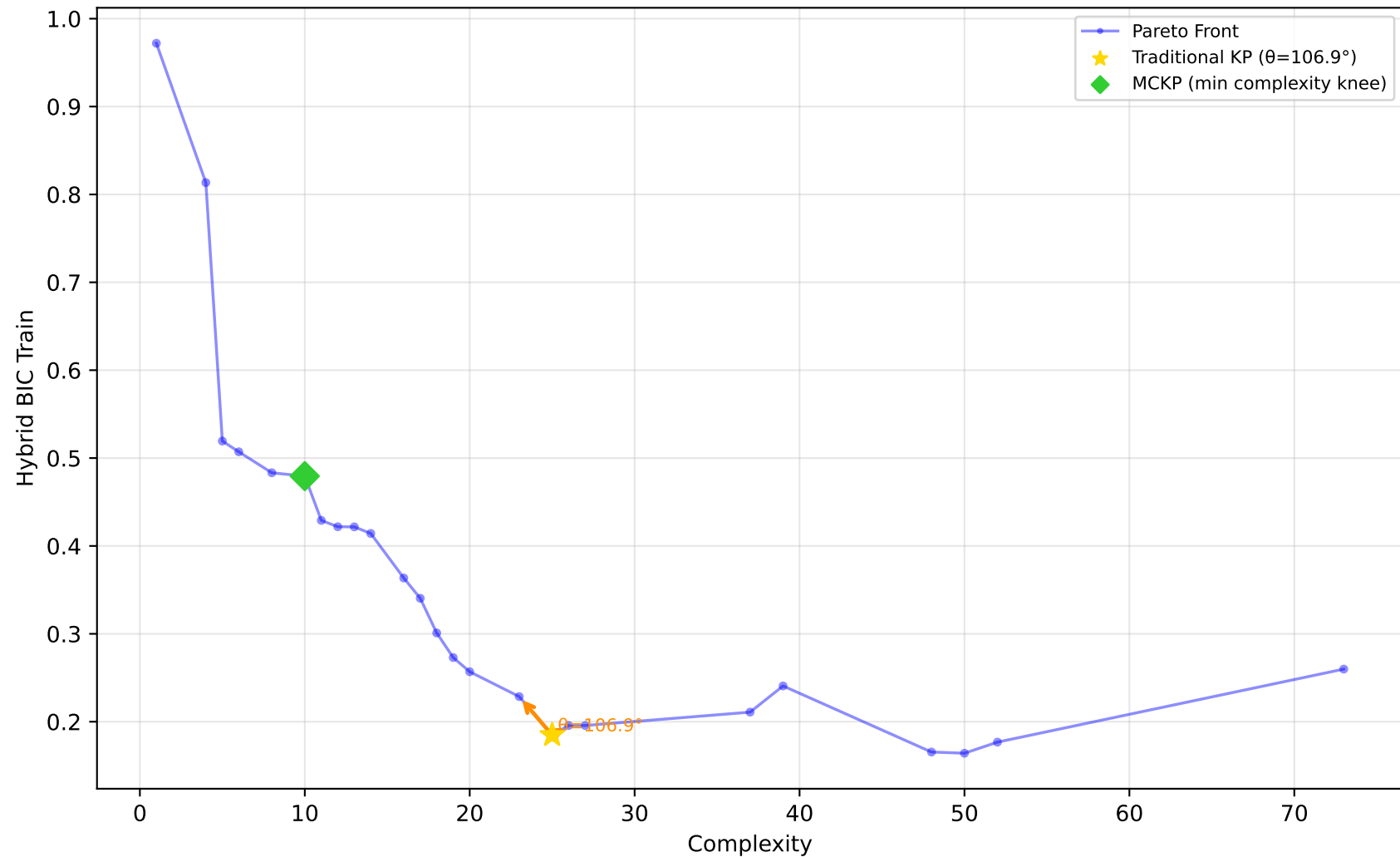
1028_SWD - Run 29 - SVP - Hybrid BIC Train \lambda_1=0.00, \lambda_2=0.60, \lambda_3=0.00 | Difficulty: 1.00 | Method: hmr
