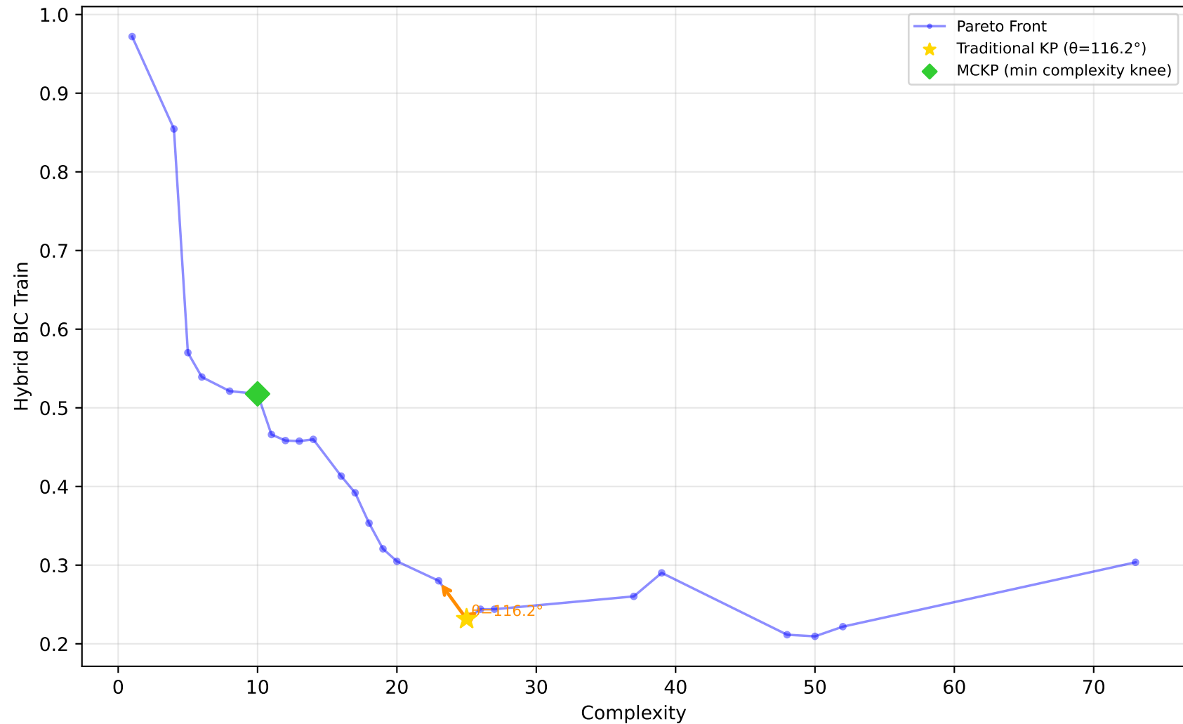
1028_SWD - Run 29 - SVP - Hybrid BIC Train \lambda_1=0.60, \lambda_2=0.00, \lambda_3=0.00 | Difficulty: 1.00 | Method: hmr
