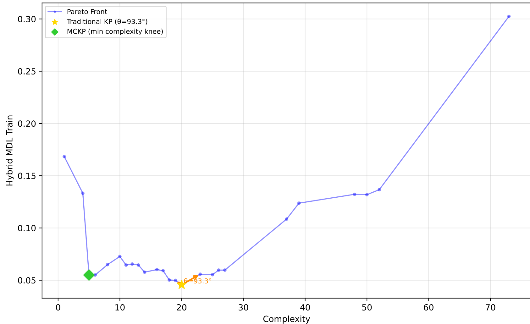
1028_SWD - Run 29 - SVP - Hybrid MDL Train \lambda_1=0.00, \lambda_2=0.60, \lambda_3=0.00 | Difficulty: 1.00 | Method: hmr
